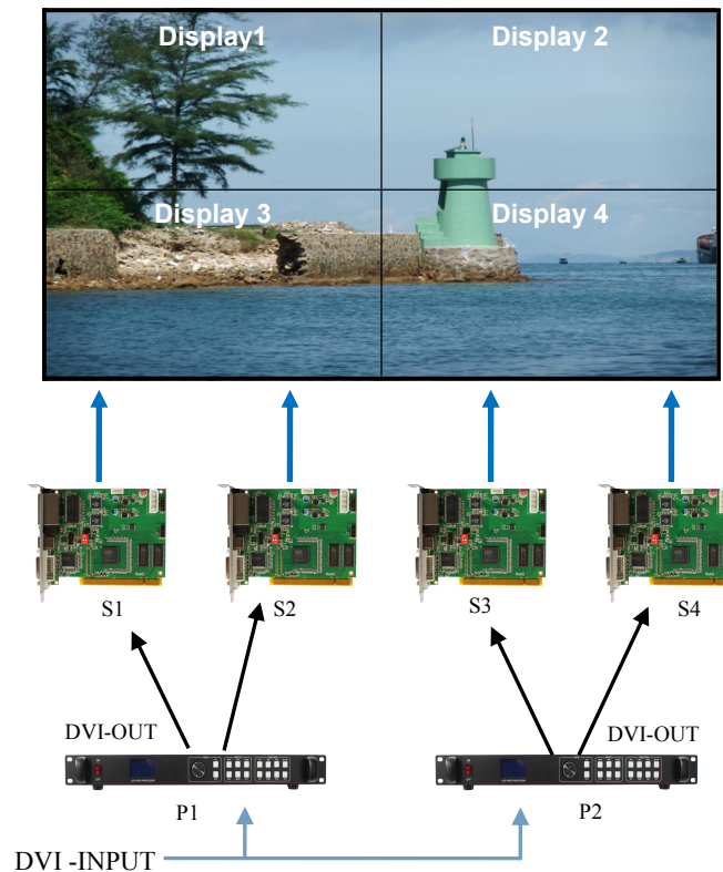
Figure 11 -Unequal Splicing
