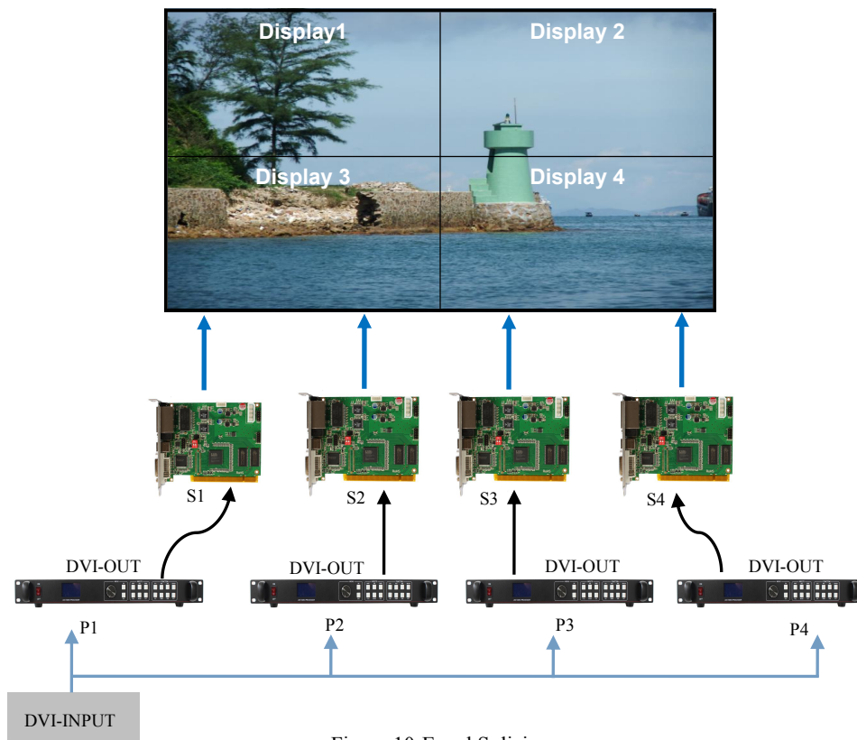
Figure 10-Equal Splicing
