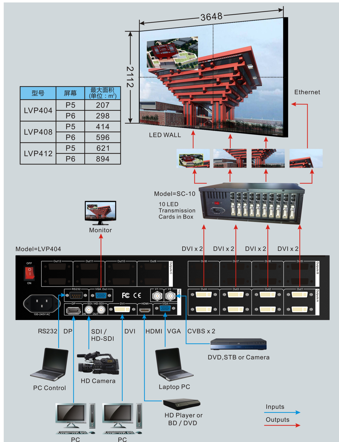
Figure 2-2 Connection diagram
