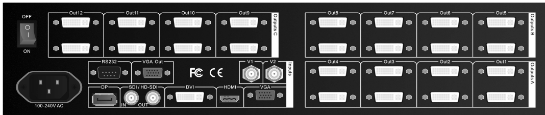
Figure 2-1 Rear view
